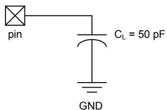
Figure 25-3. Load Conditions
