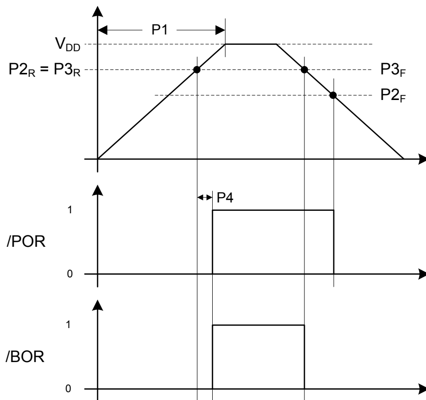
Figure 25-6. Power-On and Brown-Out Reset and Voltage Parameters
