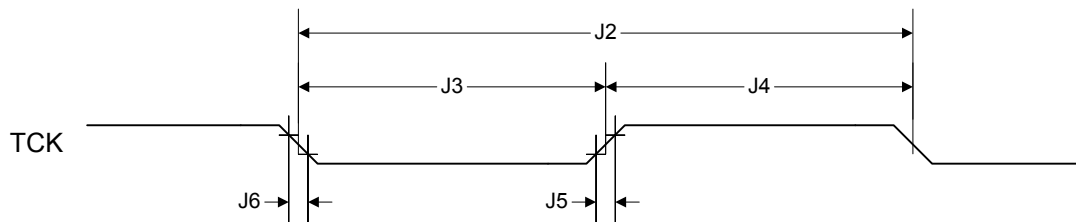
Figure 25-4. JTAG Test Clock Input Timing
